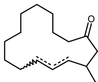
5-Cyclopentadecen-1-one, 3-methyl-
